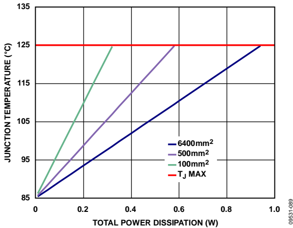
Figure 89. Junction Temperature vs. Power Dissipation, T A = 85°C
